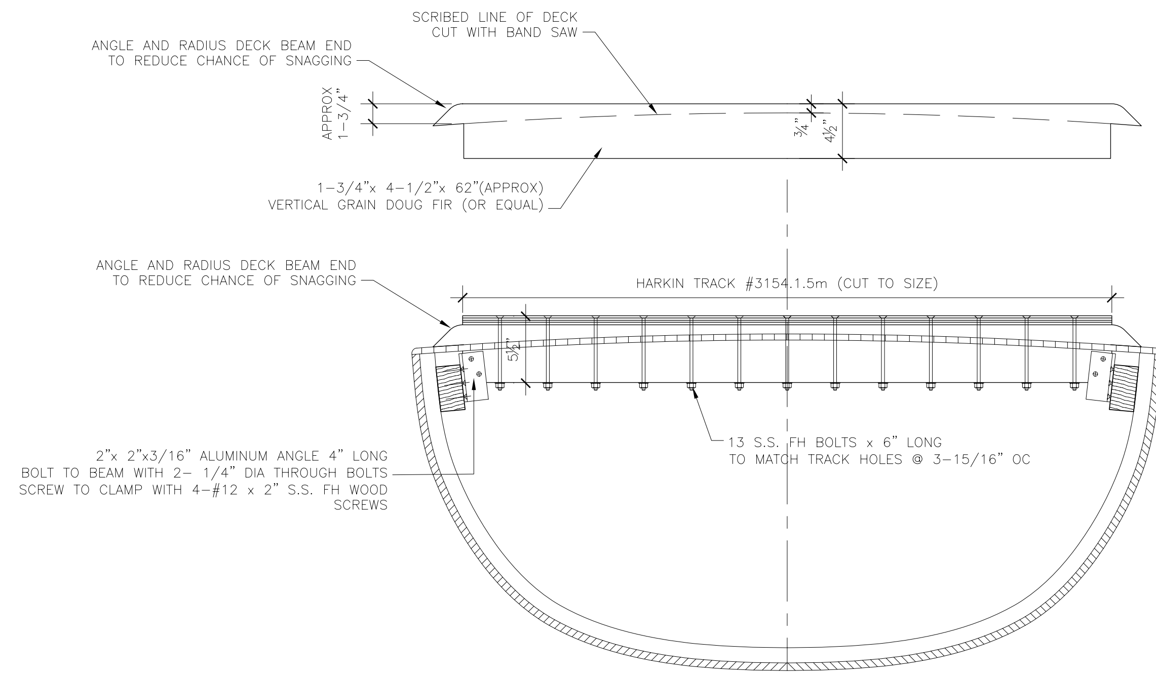
SECTION WITH BEAM Scale 1-1/2" = 12"
