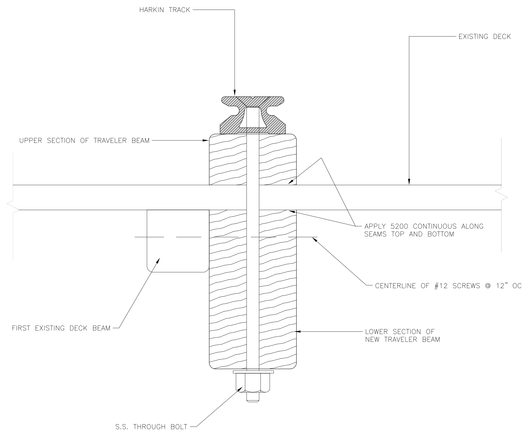
TRAVELER TRACK SECTION- WOOD BOATS Full Scale
