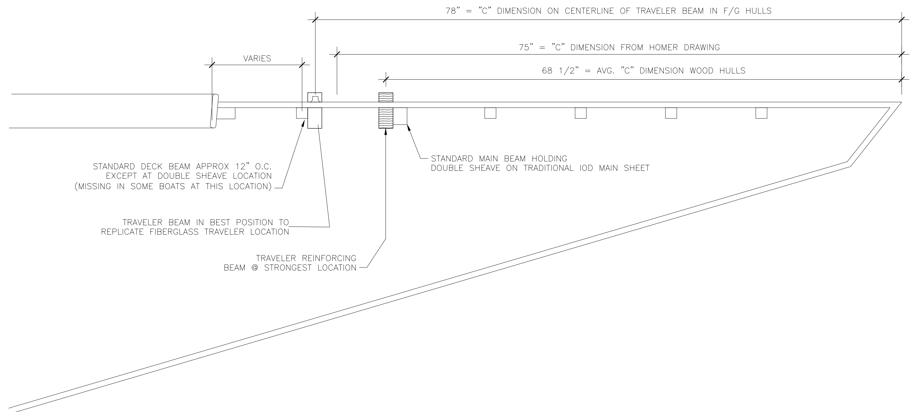
WOOD AFT SECTION WITH COMPARABLE "C" DIMENSIONS Scale 1-1/2" = 12"
