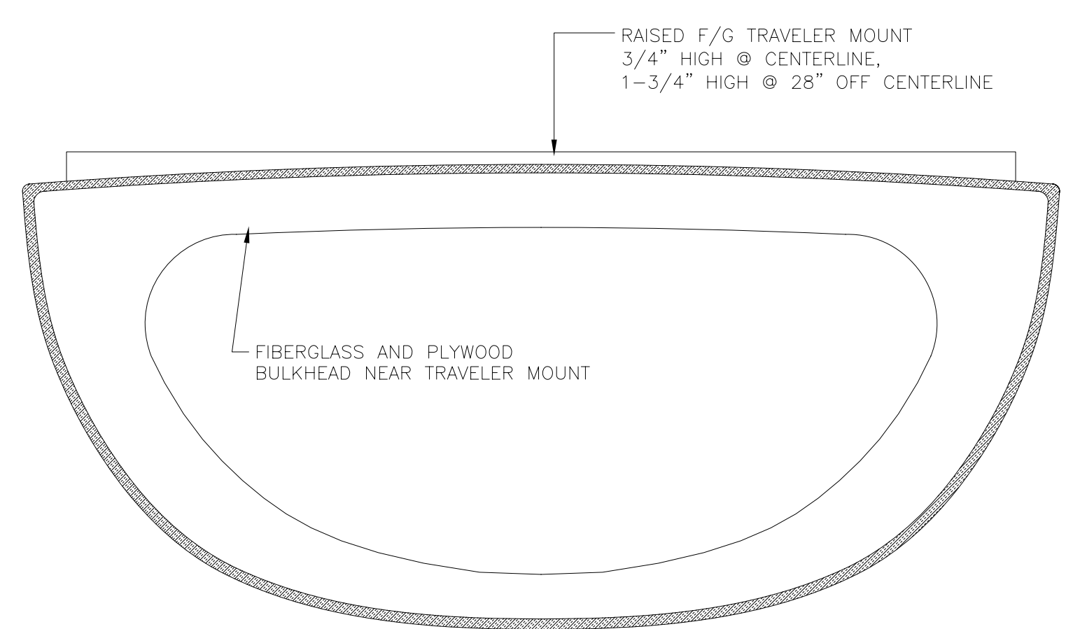
F/G SECTION @ TRAVELER Scale 1 1/2" = 12"
